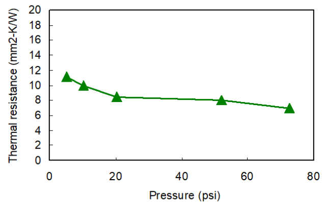
X-23-7783D Pressure vs. Thermal resistance
