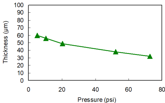
X-23-7783D Pressure vs. Thickness
