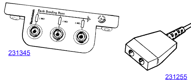
Figure 1. Typical common point grounds
