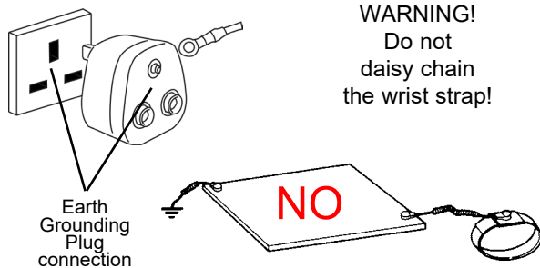
Figure 13. Equipment grounding using an EBP Plug
