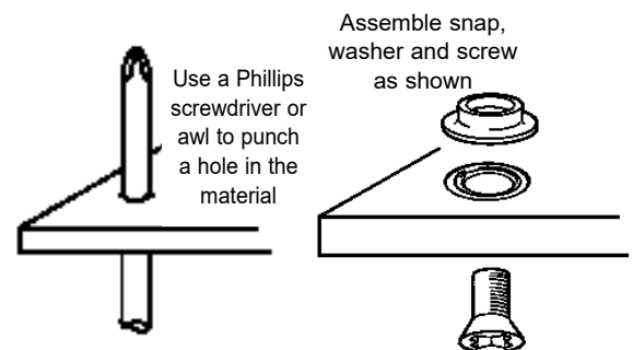
Figure 8. Installing screw-on mat grounding snap
