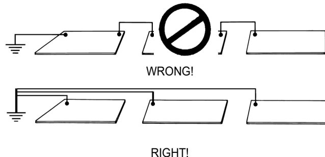
Figure 3. ESD mats should never be grounded in series, i.e. daisy chained
