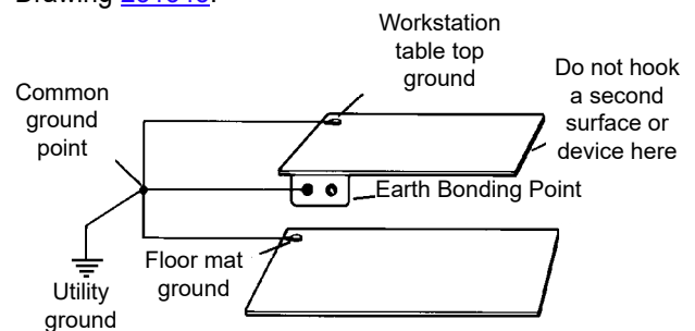
Figure 11. Earth Bonding Point installation
