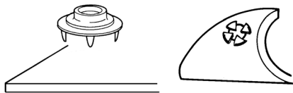
Figure 9. Installing push and clinch mat grounding snap
