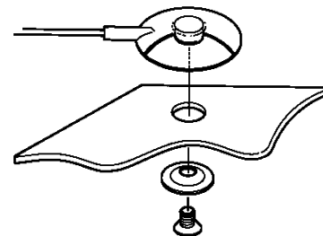
Figure 12. Installing 231280 to mat using supplied hardware
