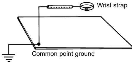
Figure 4. Common point ground for each workstation
