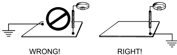
Figure 5. Proper grounding of wrist straps
