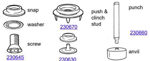
Figure 7. Three kinds of snaps
